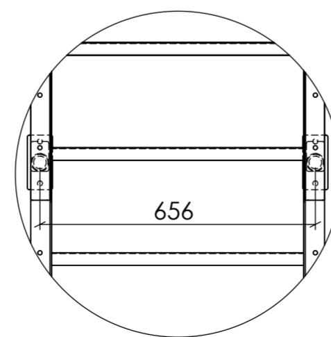
DETAIL N SCALE 2 : 25
